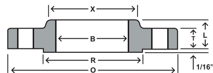
SLIP—ON
