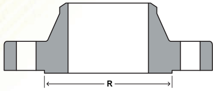
RAISED FACE
